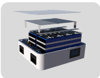
51.2V100Ah/25.6V200Ah (Internal View)
