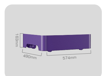
51.2V100Ah/25.6V200Ah (Base sizes)
